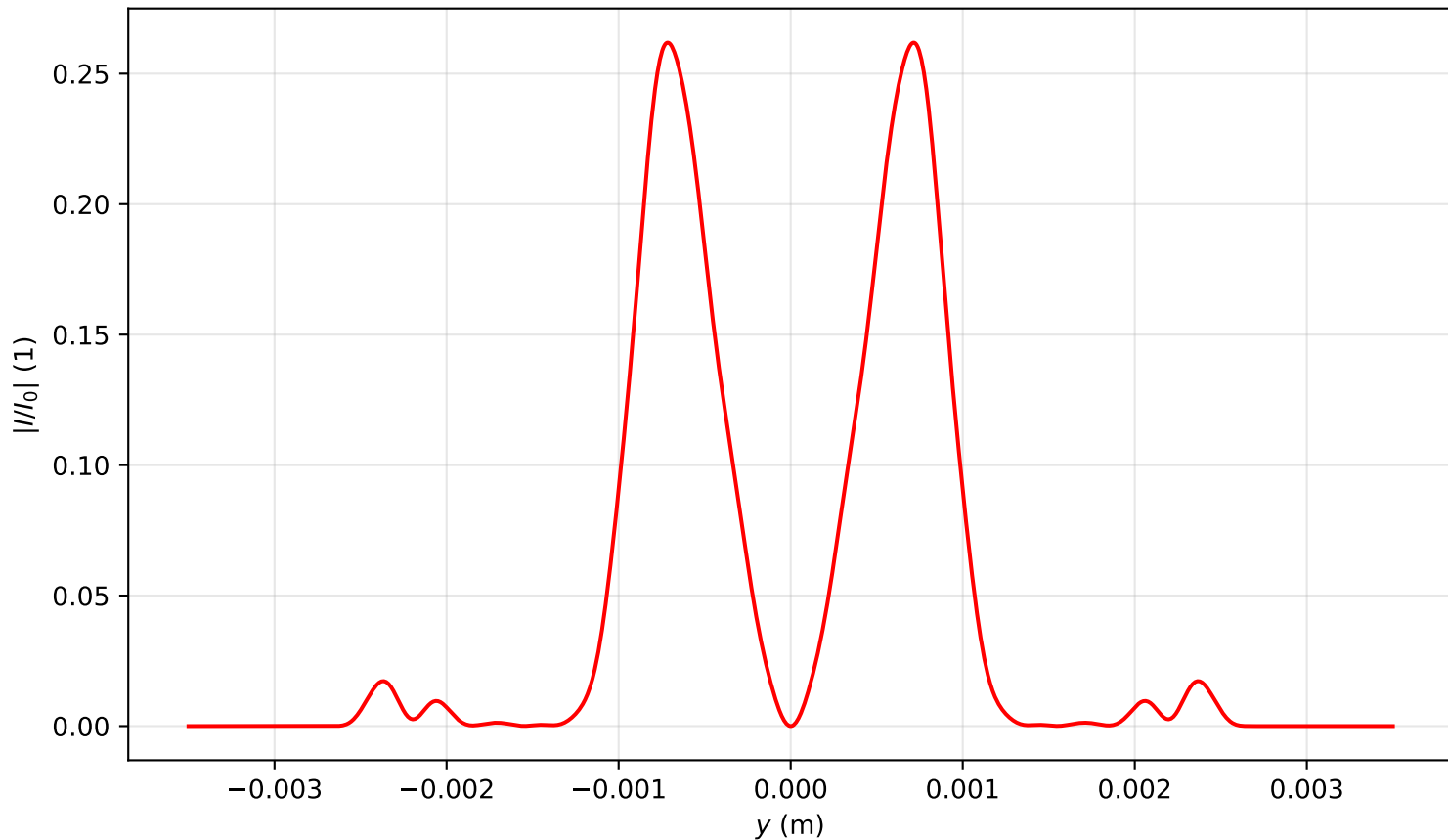
Intensity profile I(x=0, y, z=2.468)/I_0 , \text{Pin}=7.0\text{Pcr} , artificial time
